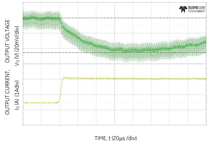
Figure 28. Transient Response to Dynamic Load Change from 50% to 100% at 12V in , C out =2x47μF+1x330μF, C Tune =6800pF, R Tune =300
