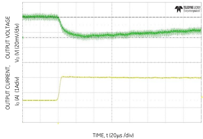
Figure 16. Transient Response to Dynamic Load Change from 50% to 100% at 12V in , C out =4x47µF+1x330µF, C Tune =15nF, R Tune =300
